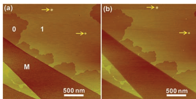
Figure 3. AFM images of graphene-templated cyclohexane adlayers. M labels the mica surface, and 0 and 1 label regions where monolayer graphene is on top of 0 and 1 adlayers of cyclohexane, respectively. Yellow arrows point to droplets. (a) A typical image of graphene-templated submonolayer cyclohexane adlayer, taken within a few hours after graphene was deposited. (b) The same area, but imaged after the sample was stored at ambient conditions for 2 months.
